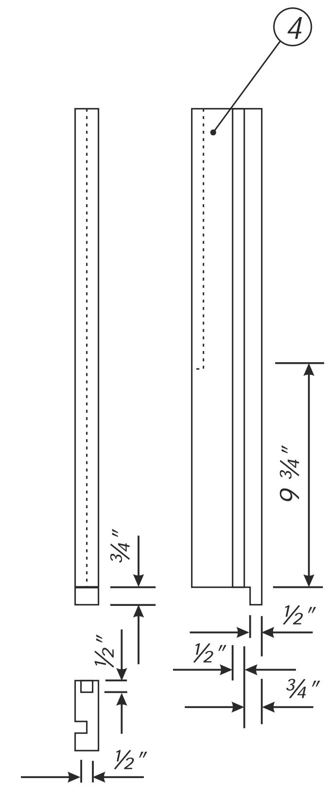
FRONT UPRIGHT
